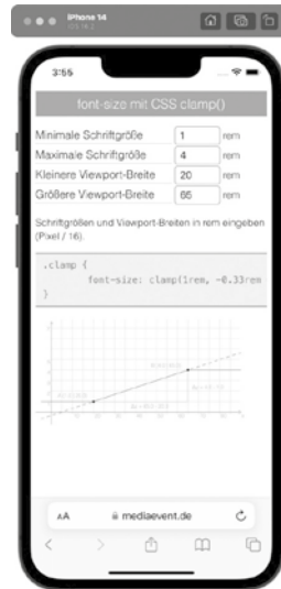
Abb. 1.6: iOS-Simulator
