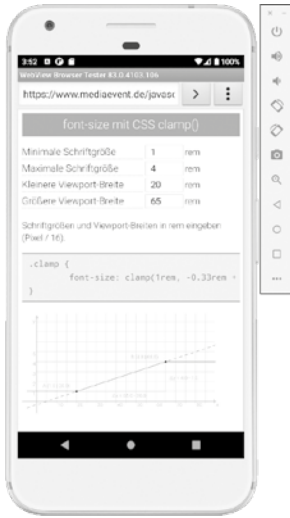
Abb. 1.5: Android-Simulator
